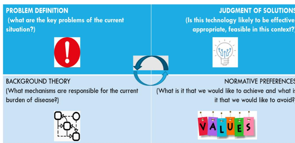
Figure 2. Interpretive frames
